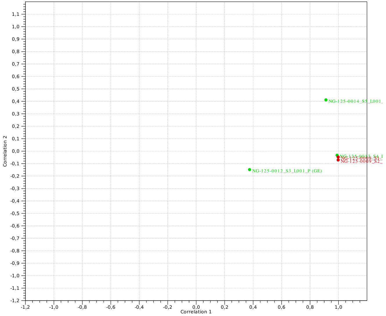
Correlation scatter plot
