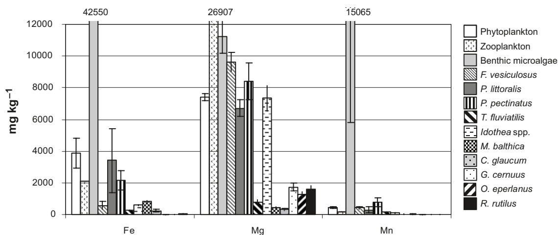
Figure 3-2. Concentration (mg kg -1 ) of Fe Mg and Mn in biota in Tixlan bay, Northern Baltic Proper; mean and SD.
